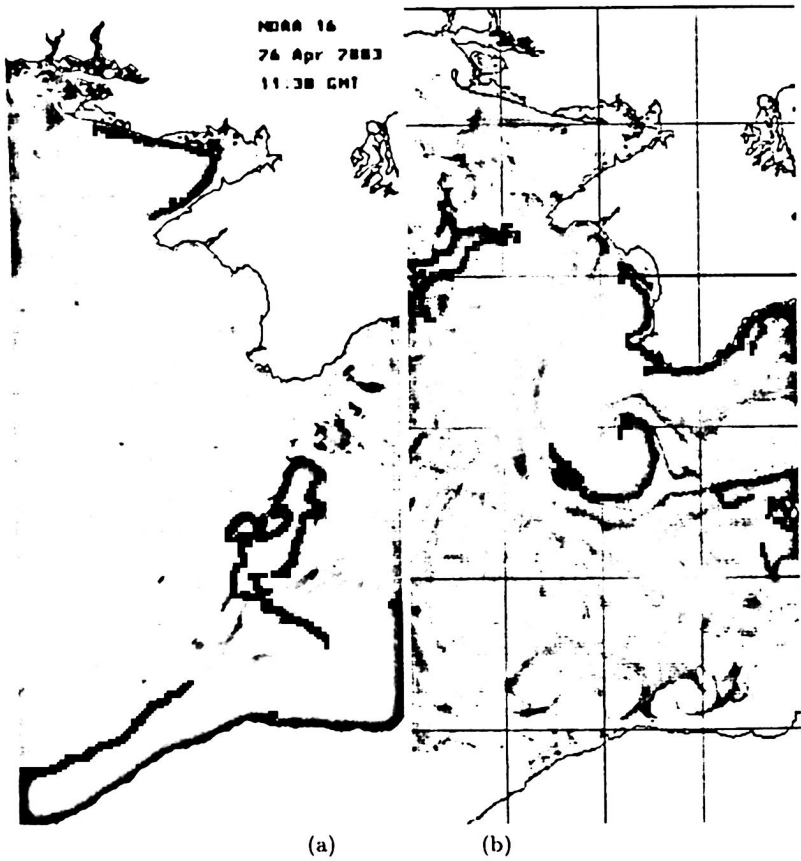
Fig. 1. Part of the Black Sea. SST computed from NOAA/AVHRR (a), SST computed from MODIS (b)
